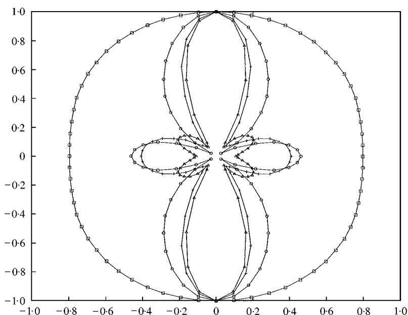
Figure 9. Directional pattern of farfield pressure from finite cylinder (CHIEF-RDT), ka = 1, 2, 2.53, 3 , b/a = 2 : \square , ka = 1 ; \circ , ka = 2 ; + , ka = 2.53 ; \triangle , ka = 3 .
