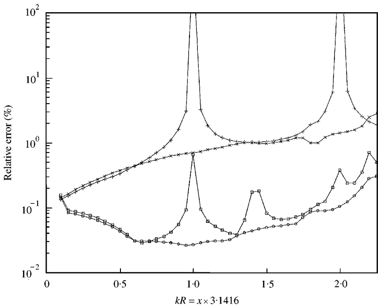
Figure 2. The maximum relative error (%) of the theoretical and calculated surface pressure by various methods for a spherical surface: +, SHF; \square , RDT; \times , CHIEF-SHF; \circ , CHIEF-RDT.
