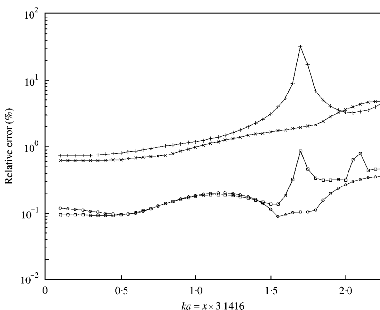
Figure 5. The maximum relative error (%) of theoretical and calculated surface pressure by various methods for a spheroid surface, b/a = 0.5 : + , SHF; \square , RDT; \times , CHIEF-SHF; \circ , CHIEF-RDT.
