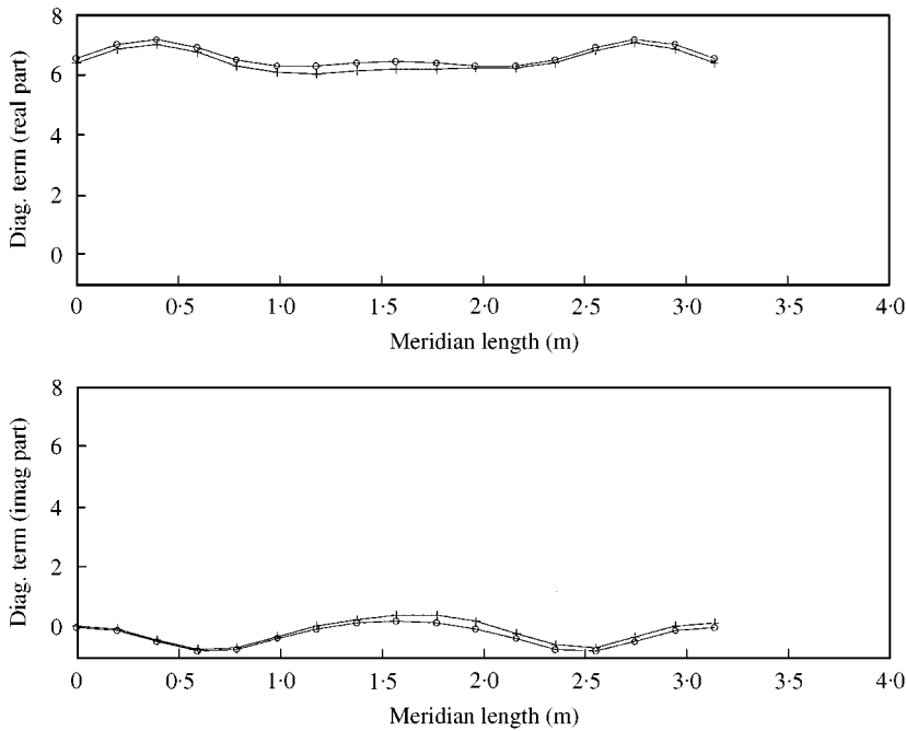
Figure 3. Diagonal terms of pressure matrix for a spherical surface calculated by SHF and RDT, kR_0 = \pi : \circ , SHF; +, RDT.
